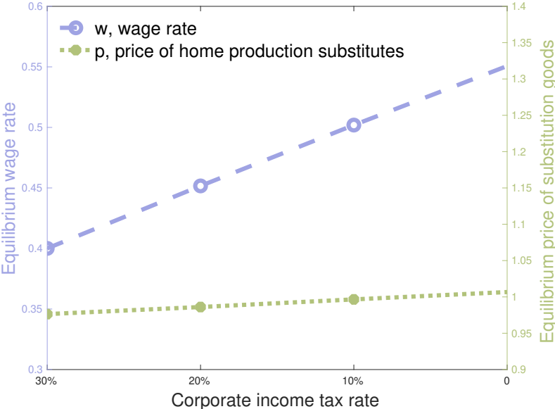
Figure 11: Equilibrium prices when \epsilon = 10
