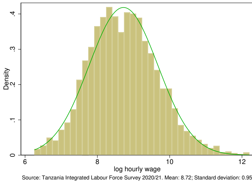
Figure 14: Distribution of log hourly wage for the working-age employees
